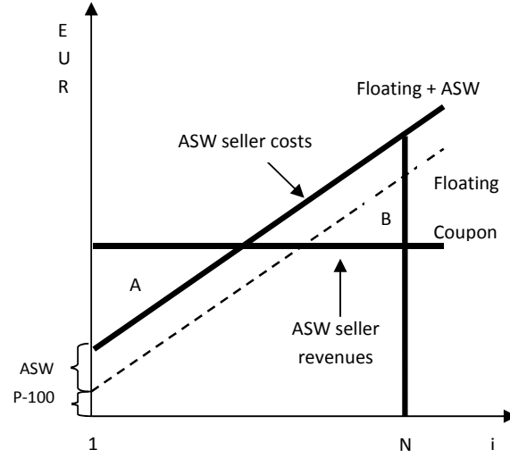
Figure 3. ASW Spreads
