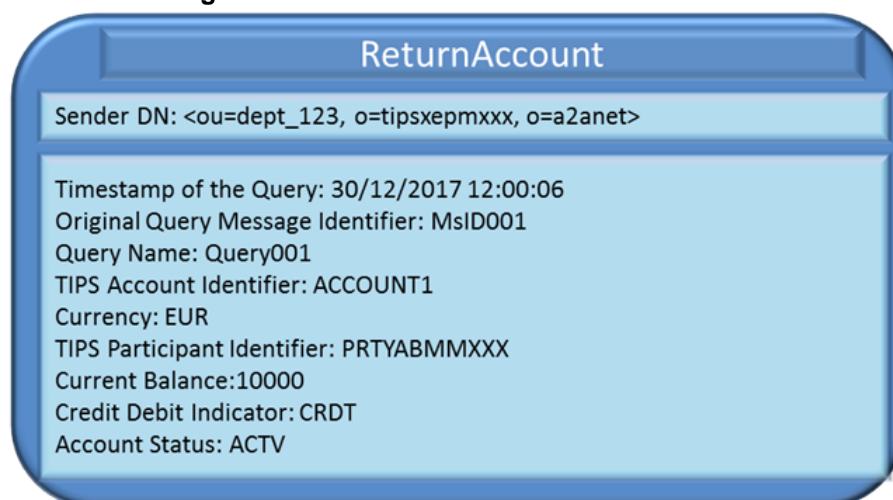
Figure 50 - Successful ReturnAccount
