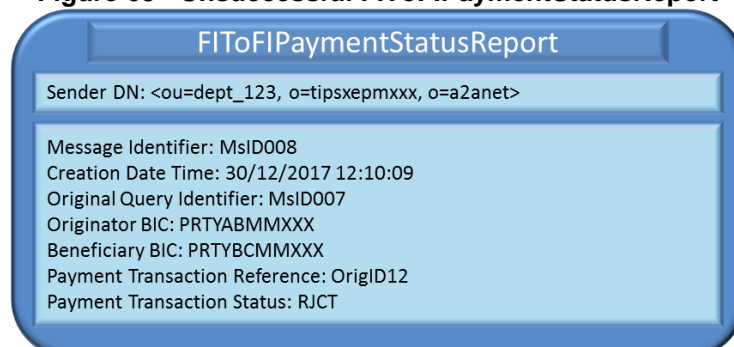
Figure 63 - Unsuccessful FIToFIPaymentStatusReport
