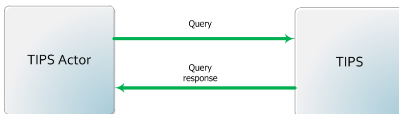
Figure 5 - Queries flow
