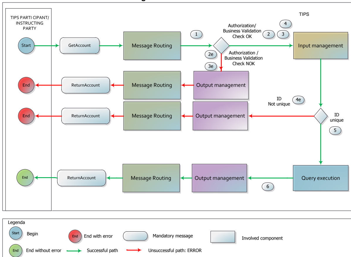
Figure 47 - Queries flow
