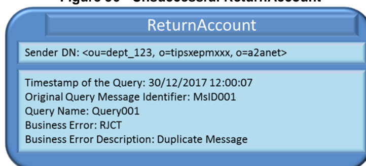
Figure 56 - Unsuccessful ReturnAccount
