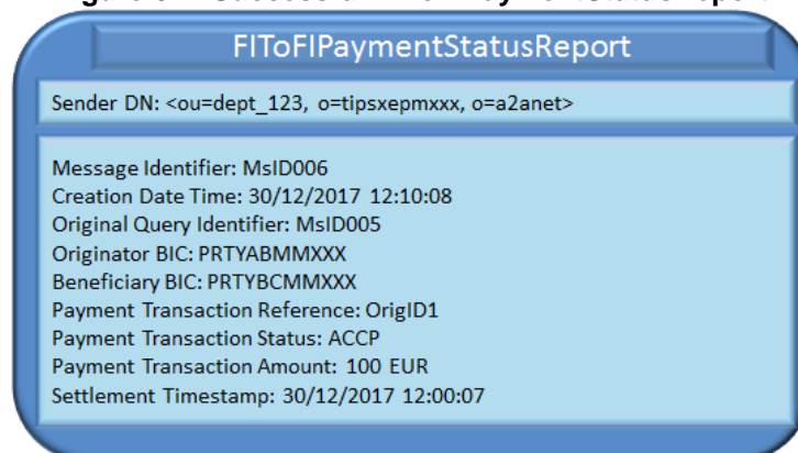
Figure 61 - Successful FIToFIPaymentStatusReport
