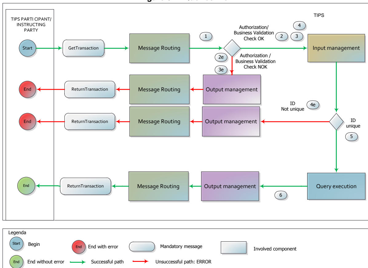
Figure 57 - Queries Flow
