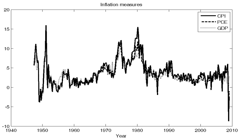
Figure 5: Inflation data
