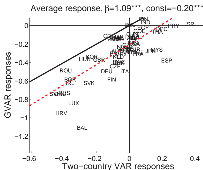
Figure 1: Differences Between Estimates of the Spillovers from US Monetary Policy Obtained from the GVAR and the Two-country VAR Models
