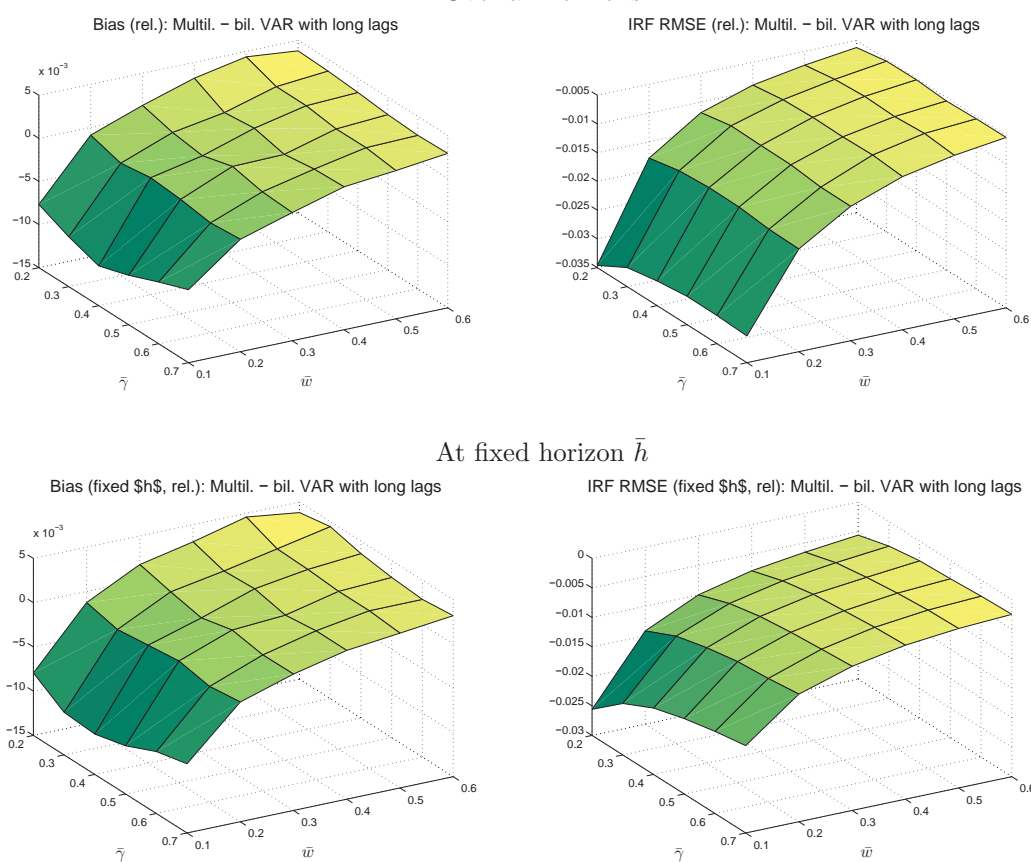
Figure 8: Difference Between Bias and RMSE of Spillover Estimates Obtained from the Multilateral Model and the Bilateral Model with Higher Lag Orders Over all horizons
