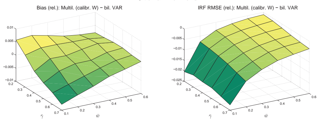
Figure 5: Difference Between Bias and RMSE of Spillover Estimates Obtained from the Multilateral with Calibrated Weight Matrix C and the Bilateral Model Over all horizons
