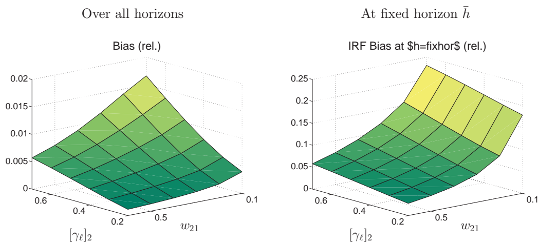
Figure 3: Asymptotic Bias in the Spillover Estimates Obtained from the Bilateral Model
