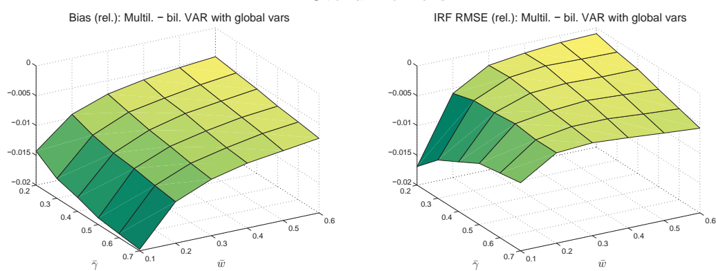
Figure 7: Difference Between Bias and RMSE of Spillover Estimates Obtained from the Multilateral Model and the Bilateral Model Augmented by Global Variables Over all horizons
